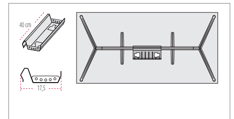
40 cm Channel for individual use 160, 180, 200 and 220 cm desks
